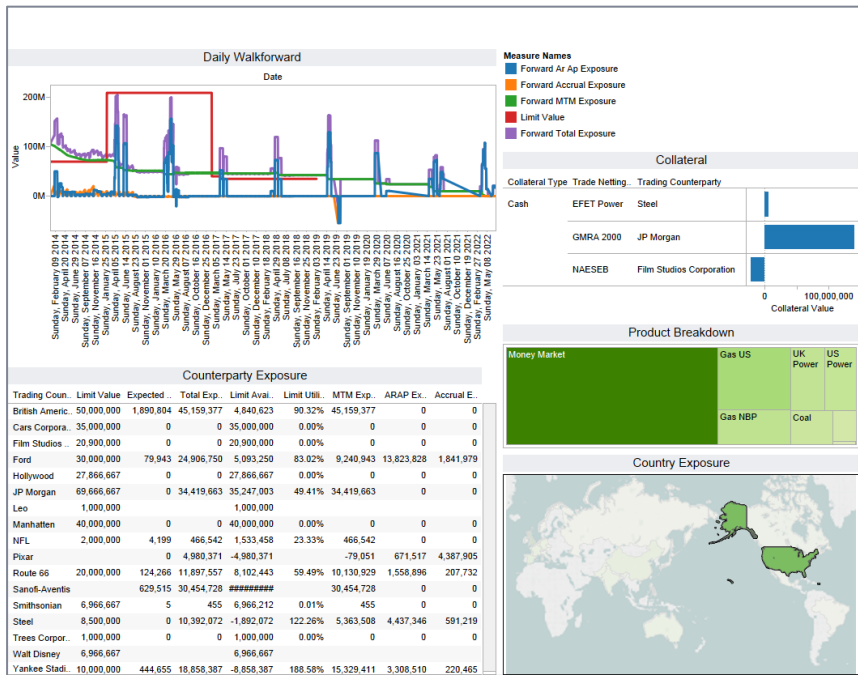
Figure 1: Credit Dashboard
